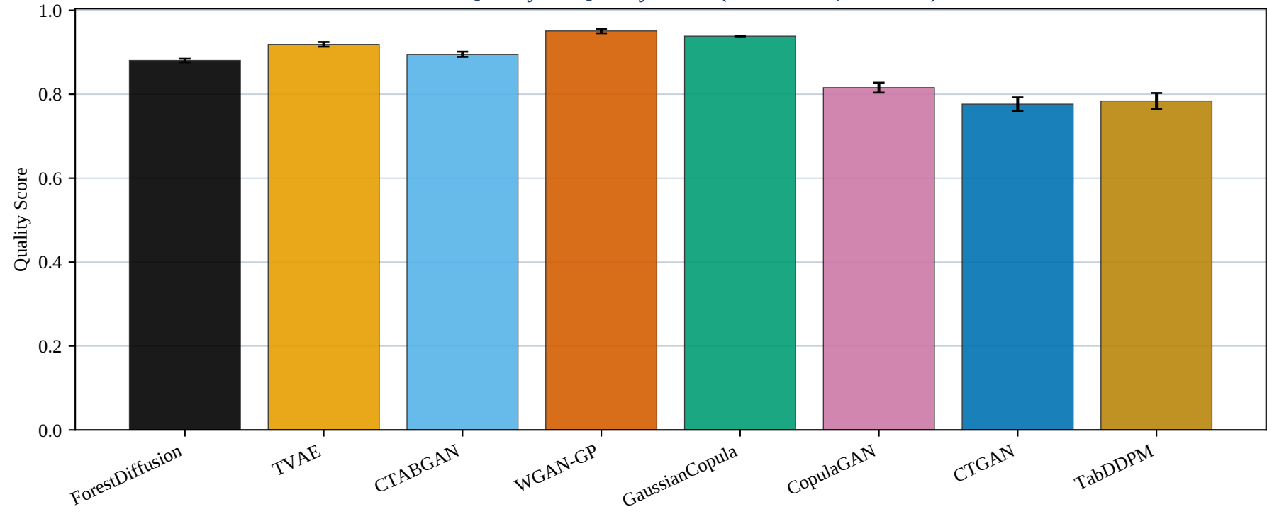
Wine Quality — Quality Score (mean \pm SD, 10 seeds)
